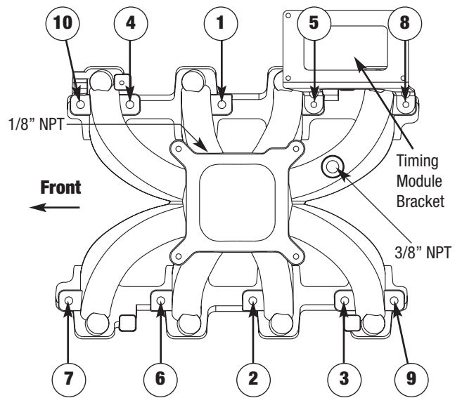
Figure 1 - Intake Manifold Tightening Sequence
